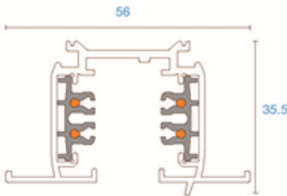
3 circuit track system
